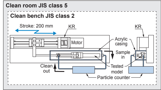
Testing device
